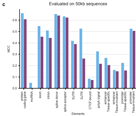
Supplementary Figure 2: Context-length extension allows to rescale SegmentNT-10kb to 100kb sequences. a) Average MCC performance across the 14 elements for the SegmentNT-10kb model with and without context-length rescaling. b-d) Performance on different input lengths without vs with context-length extension.
