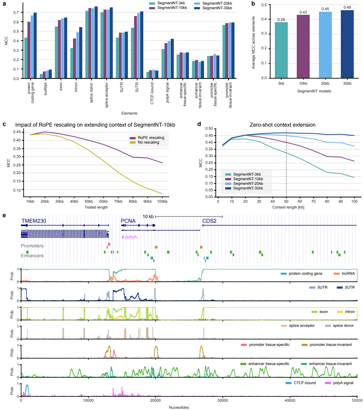
Figure 3: Adaptation and zero-shot generalization of SegmentNT across multiple sequence lengths. a) Performance of SegmentNT trained on 3kb, 10kb, 20kb and 30kb sequences on 14 types of genomic elements. We used as metric the MCC. b) Average MCC performance of the different models across the 14 elements. c) Context-length extension through Rotary Position Embedding (RoPE) rescaling allows to improve performance of SegmentNT-10kb on up to 100kb sequences. Average MCC performance across the 14 elements for the SegmentNT-10kb model with and without context-length rescaling. d) Long-range models improve generalization on longer contexts while maintaining performance on shorter contexts. Average MCC performance across the 14 elements for the different SegmentNT models per input sequence length. e) Representative example of annotations and predicted probabilities of the 14 types of genomic elements for a 50kb region at the TMEM230/PCNA/CDS2 gene locus located in the test set. Gene isoforms with respective exons and introns, as well as promoter and enhancer regulatory elements are shown.
