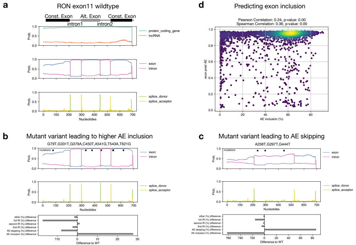
Supplementary Figure 4: Prediction of sequence variants affecting splicing isoforms. a ) SegmentNT prediction of gene elements of RON exon11 minigene wildtype sequence. b-c ) SegmentNT prediction for a minigene variant leading to (b) higher exon inclusion and (c) higher exon skipping. Predictions for exon/intron (top) and splice sites (middle) are shown. Nucleotide mutations in each minigene variant are shown with black stars. Bottom bar-plot shows the experimental differences in isoform abundance relative to the wildtype minigene sequence. d ) Scatter-plot comparing SegmentNT's exon prediction and the inclusion of the alternative exon 11 (AE) across all minigene variants. Pearson and Spearman correlation coefficients and p-values are shown.
