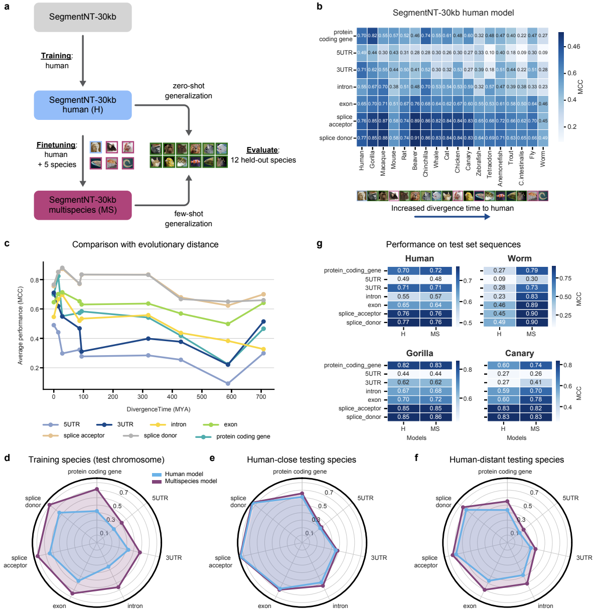
Figure 5: SegmentNT generalizes across species. a) Cartoon explaining zero-shot and few-shot specie generalization of SegmentNT. SegmentNT-30kb-multispecies was trained on genic elements from human plus 5 additional species. Both human (zero-shot) and multispecies (few-shot) models were evaluated on a held-out test set of 12 species. b) Performance of the human model on the gene elements of all species, sorted by divergence time to human. We used as metric the MCC. c) Comparison between MCC performance and divergence time per gene element. The MCC was averaged for species with the same evolutionary distance. d-f) Radar plot depicting the performance of the human and multispecies SegmentNT models per element for (d) species in the training set, (e) human-close species in test set, and (f) human-distant species in test set. g) Performance of the human (H) and multispecies (MS) model per element for 4 representative species.
