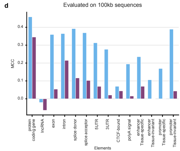
Supplementary Figure 2: Context-length extension allows to rescale SegmentNT-10kb to 100kb sequences. a) Average MCC performance across the 14 elements for the SegmentNT-10kb model with and without context-length rescaling. b-d) Performance on different input lengths without vs with context-length extension.
